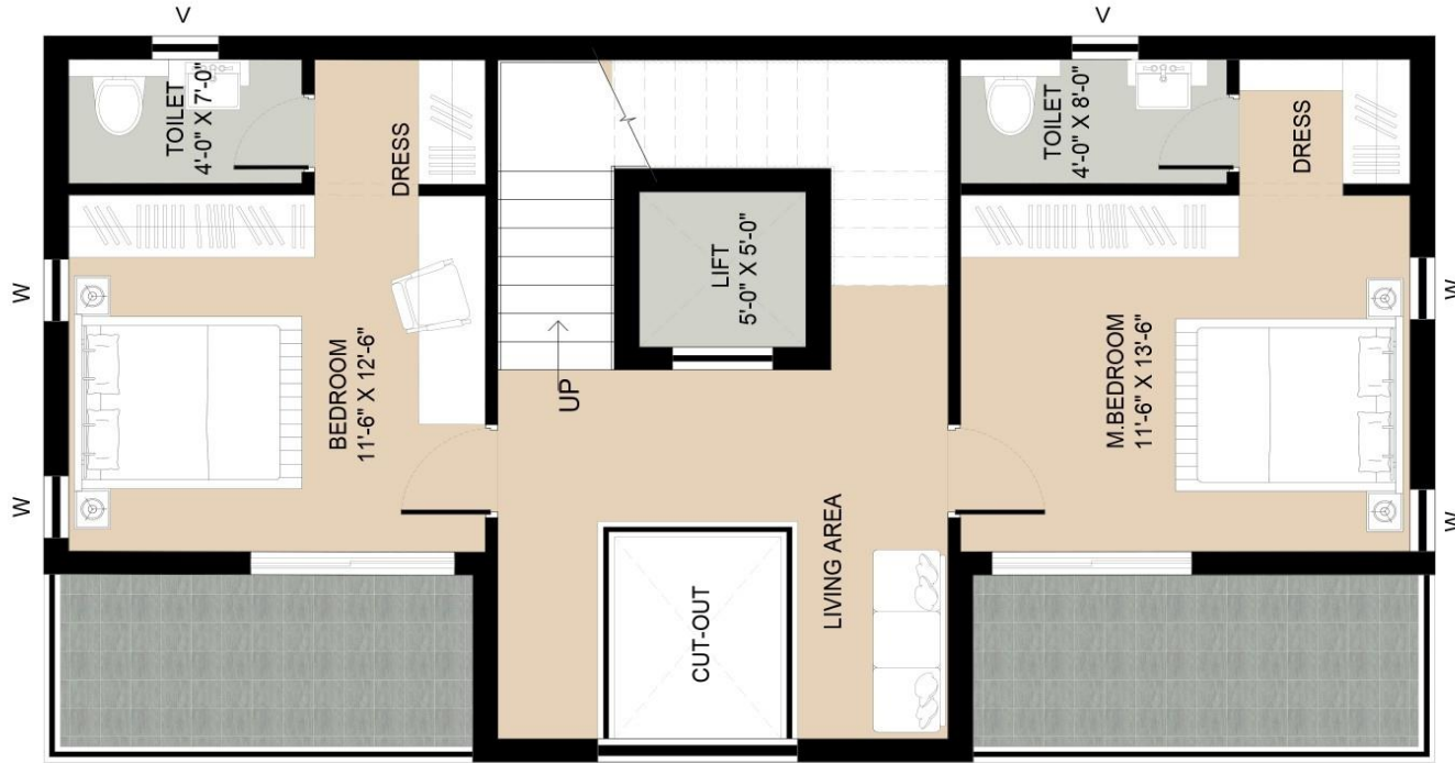
FIRST FLOOR FLOOR BUILT-UP AREA - 975 SFT
