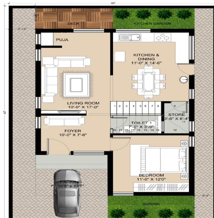
(30' X 45') WEST 150 SQYD DUPLEX
